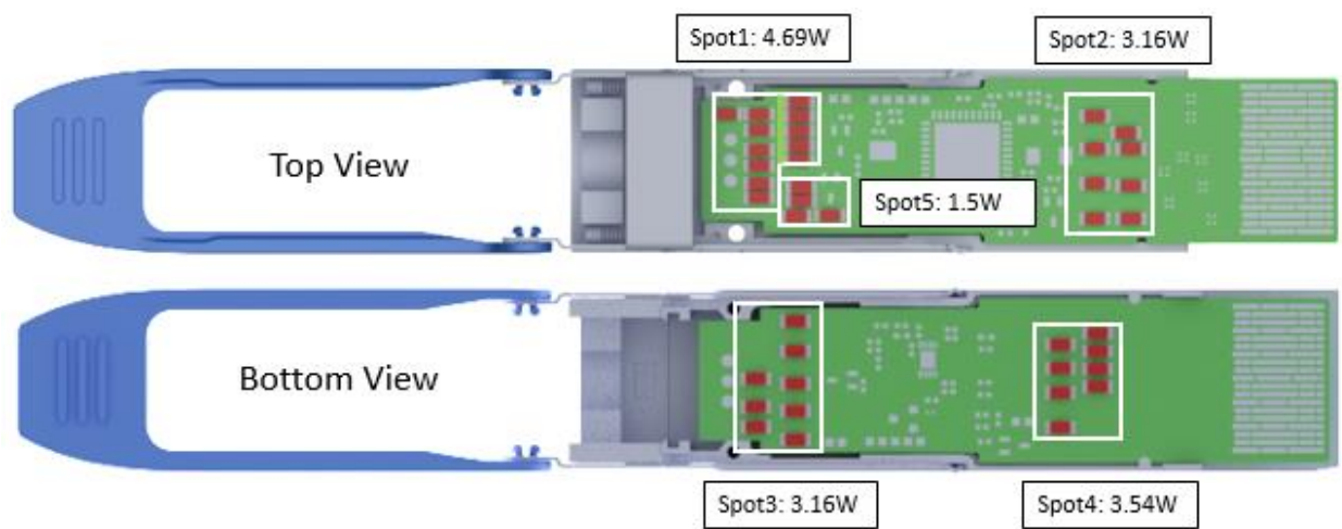
Figure 6: Thermal spots distribution
