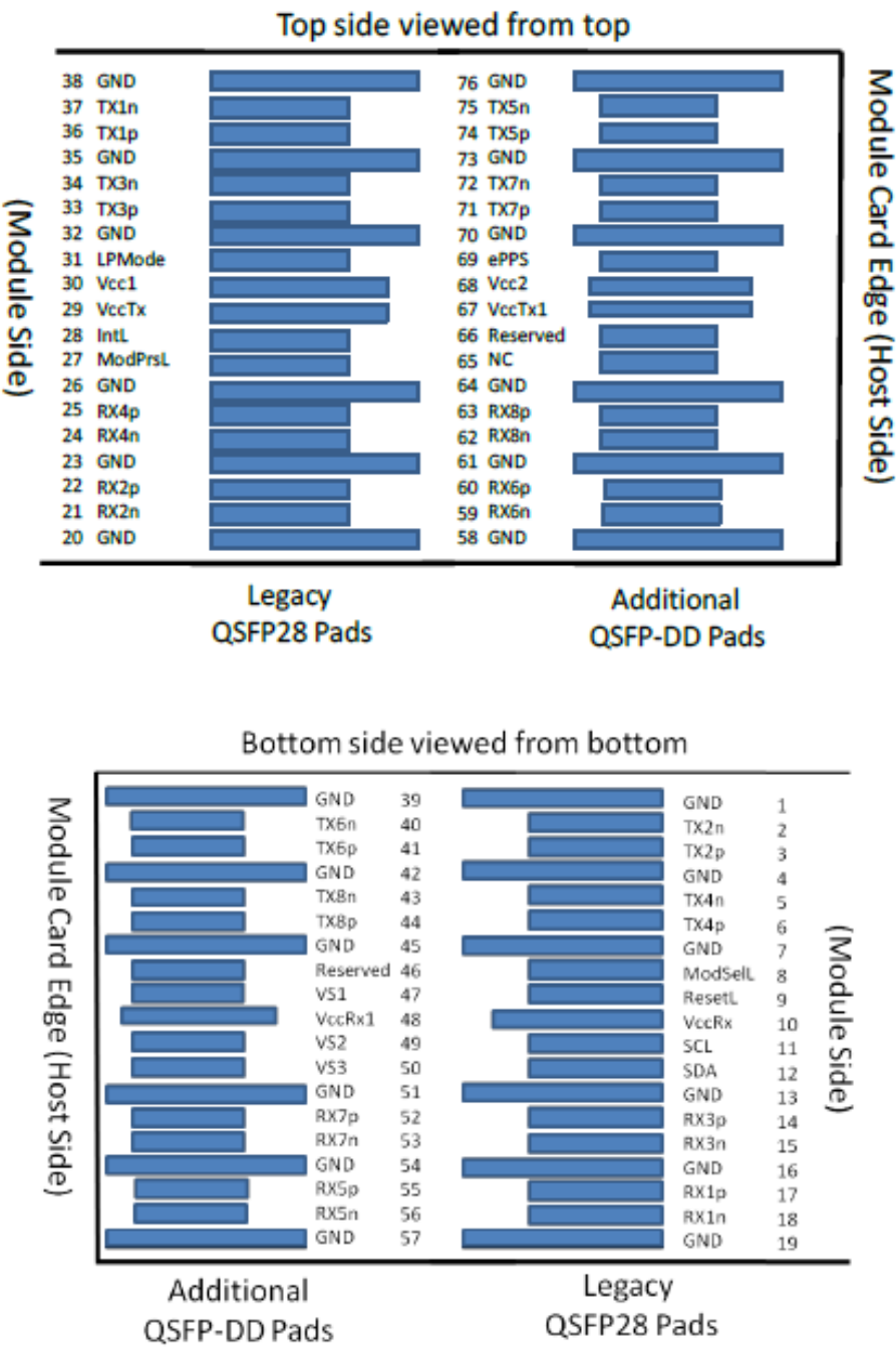
Figure 9: QSFP-DD Module Pad Layout
