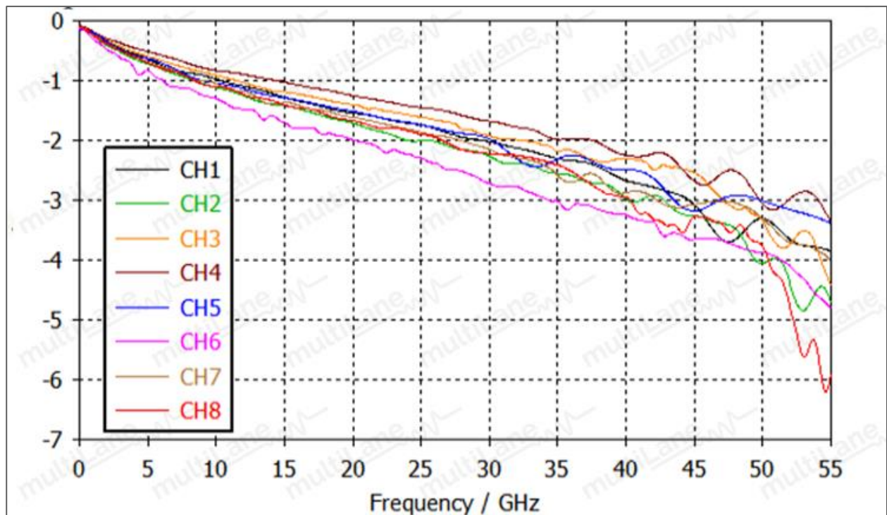
Figure 8: Insertion Loss Graph
