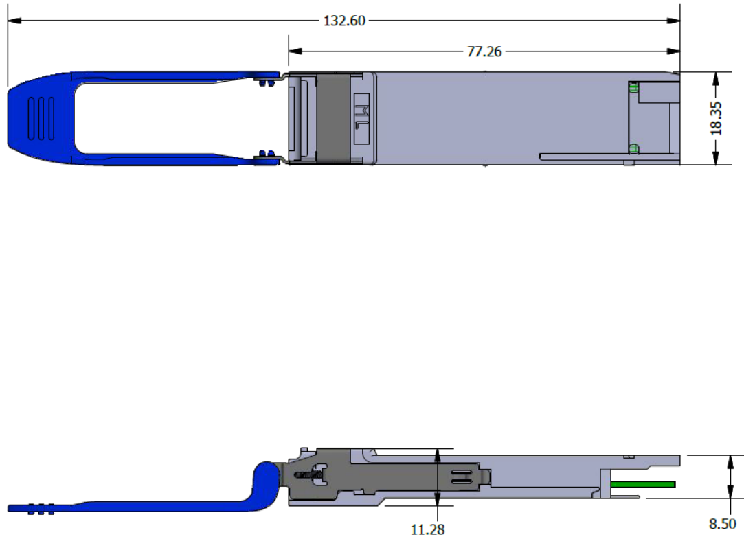
Figure 10: Mechanical Dimensions
